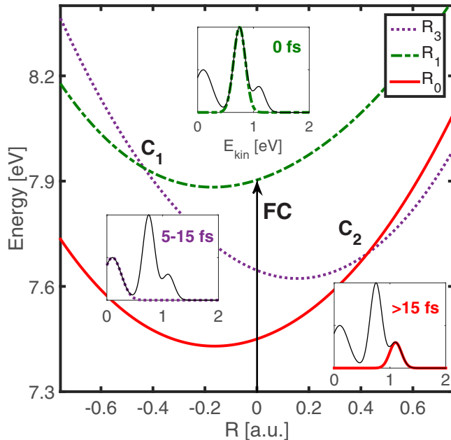
FIG. 1. One-dimensional neutral potentials along the wagging mode of \text{CH}_2 with energy measured relative to the neutral ground state. The diabatic states shown are coupled via coupling elements of Gaussian shape with a strength of 0.082 eV and a FWHM of 0.6 a.u. (see [24] for further details). The first nonadiabatic crossing, C_1 , is reached in about 5 fs. The second crossing, C_2 , is reached in 15–20 fs. (Insets) Cartoons of the expected photoelectron spectra due to ionization at several critical time delays are shown. The black line is the total photoelectron spectra with contributions from all ionic states integrated over time.
