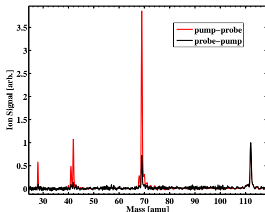
Figure 5.4: Time of flight mass spectra of uracil for negative and positive time delays (+/- 200 fs). Both spectra are normalized to the parent ion yield.
