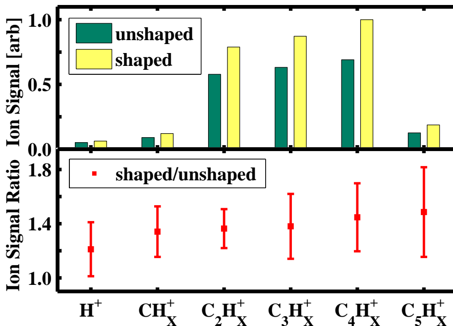
Figure 3.5: Top panel: peak integrals with the unshaped and the shaped pulse (UV background subtracted), Bottom panel: shaped/unshaped peak integral ratios.
