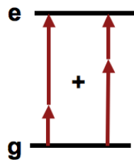
Figure 1.1: Interference between two quantum excitation paths. By changing the relative phase between the photons in each path, the total excitation to the excited state e can be controlled.
